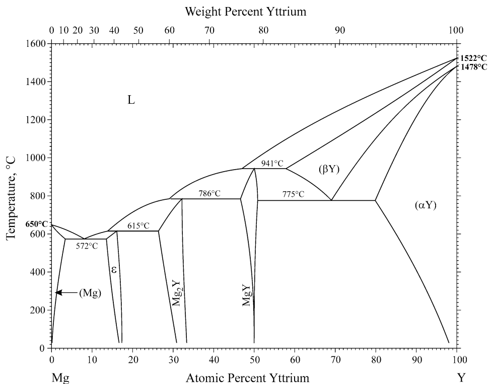
Fig. 1 Mg-Y phase diagram
